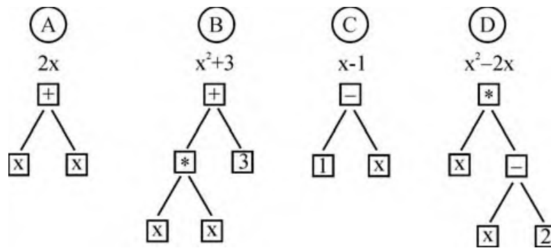
Figure 7.12 Population of four polynomial functions.
