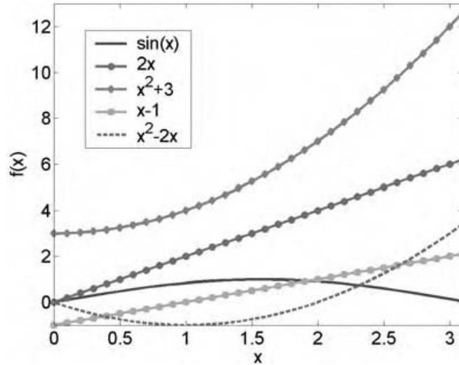
Figure 7.13 Plots of chromosomes approximating \sin(x) .
