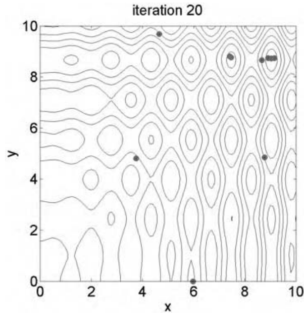
Figure 7.7 Swarm after 20 iterations.
