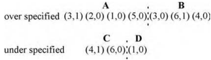
Figure 5.28 Crossover with the mGA.
