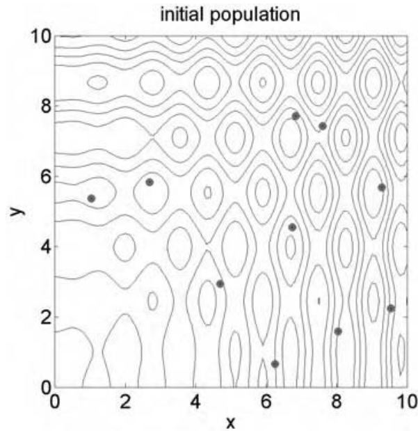
Figure 7.3 Initial random swarm of 10 particles.
