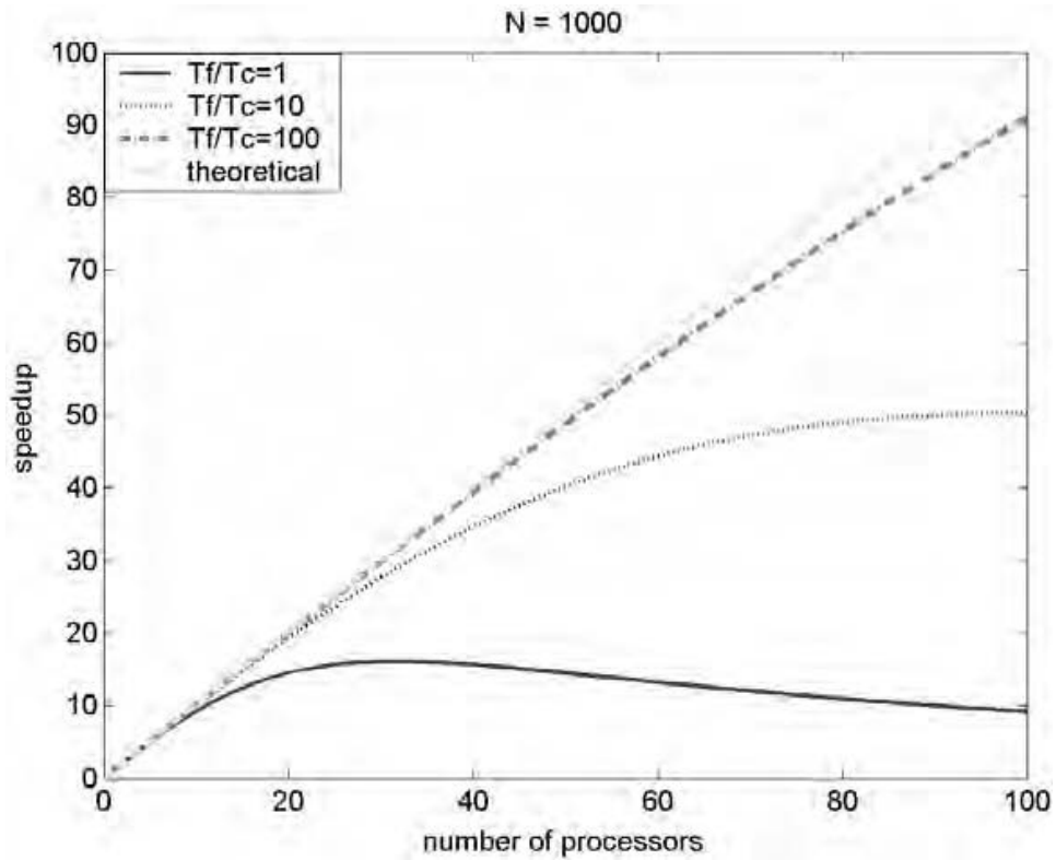
Figure 5.32 Theoretical speedup of GA with N_{pop} = 1000 .
