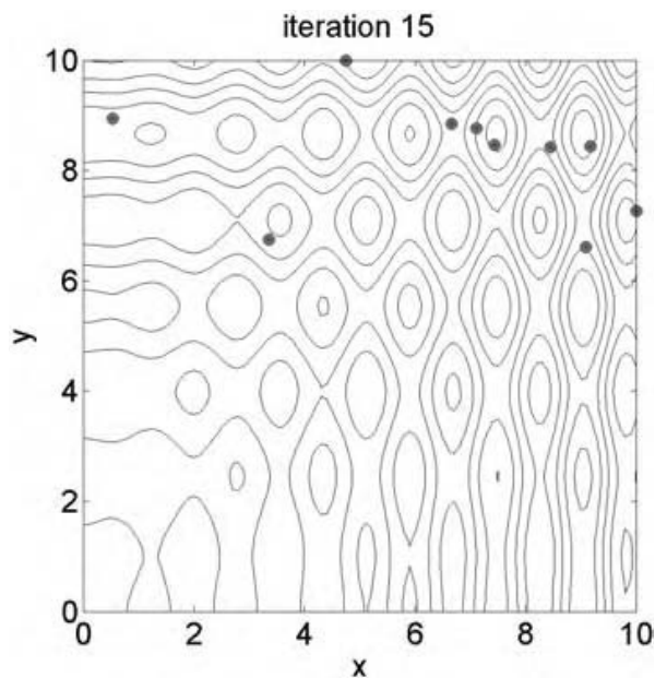
Figure 7.6 Swarm after 15 iterations.
