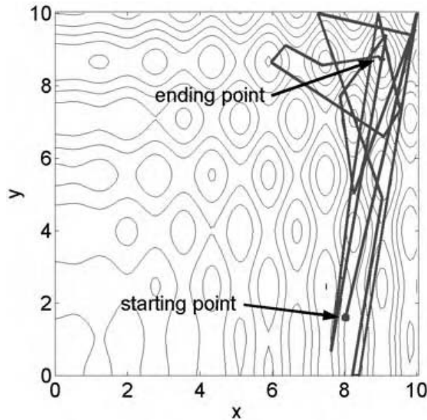
Figure 7.9 Path taken by a single PSO particle.
