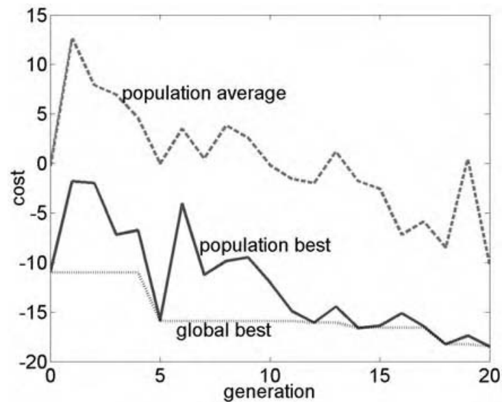
Figure 7.8 Convergence of the PSO algorithm.
