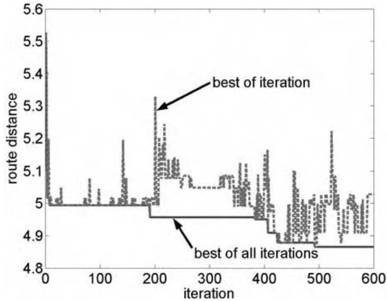
Figure 7.11 ACO convergence of the traveling salesperson problem.
