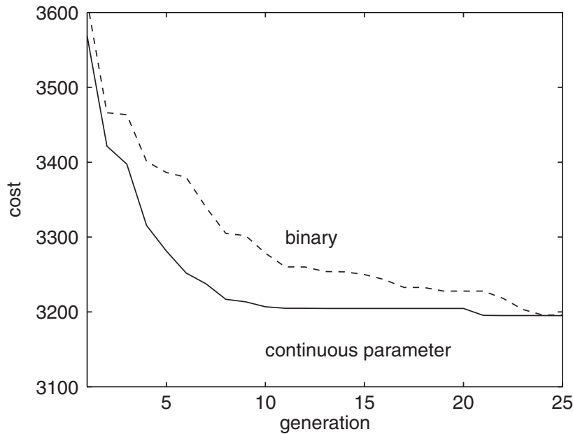
Figure 4.13 Plot of the minimum of the population as a function of generation for the binary genetic and continuous parameter GAs applied to the emergency response unit problem. These results were averaged over 20 different runs.
