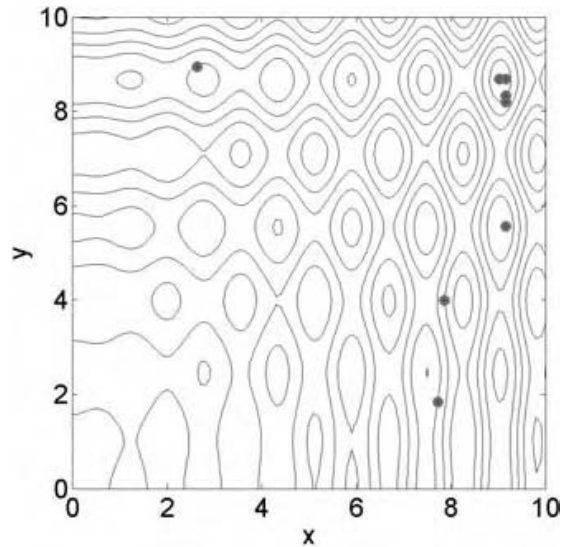
Figure 3.5 Contour plot of the cost function with the population after the third and final generation.
