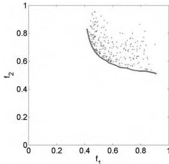
Figure 5.3 Final population and Pareto front found by the GA.
