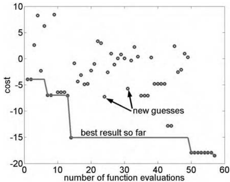
Figure 7.2 Convergence of the SA.
