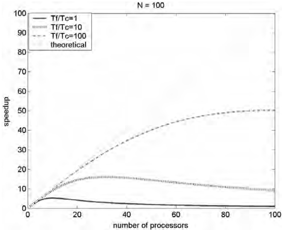
Figure 5.31 Theoretical speedup of GA with N_{pop} = 100 .
