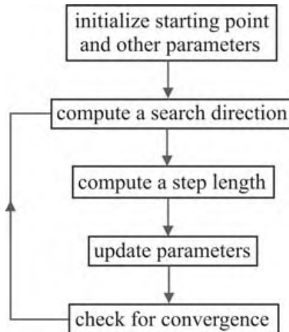
Figure 1.10 Flowchart for a typical line search algorithm.
