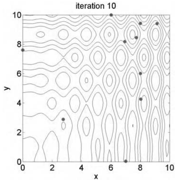
Figure 7.5 Swarm after 10 iterations.
