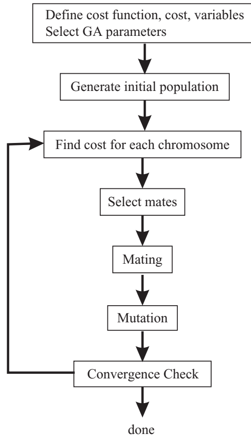
Figure 3.1 Flowchart of a continuous GA.
