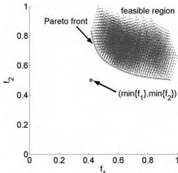
Figure 5.1 Solutions to the MOO problem in (5.1). The Pareto front is the line formed by the optimal solutions. The point formed by the minimum of both functions separately is labeled.
