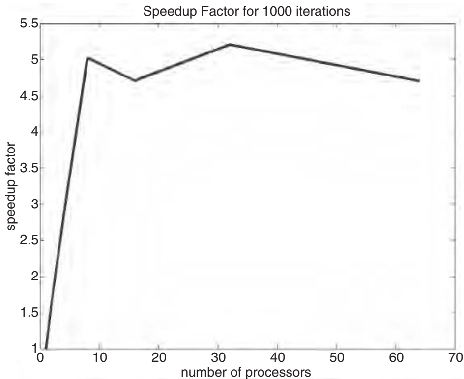
Figure 5.34 Speedup curve for example parallel GA problem.
