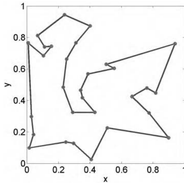
Figure 7.10 ACO solution to 30 city traveling salesperson problem.
