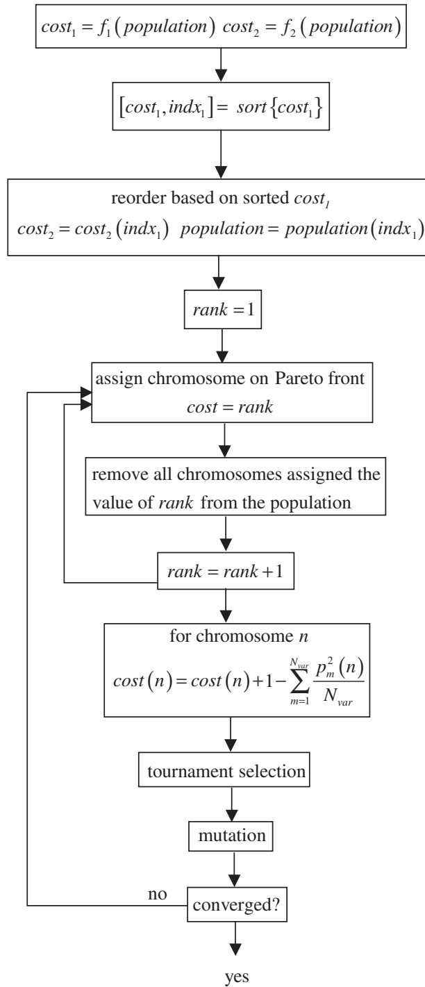
Figure 5.2 Flowchart of the Pareto GA.
