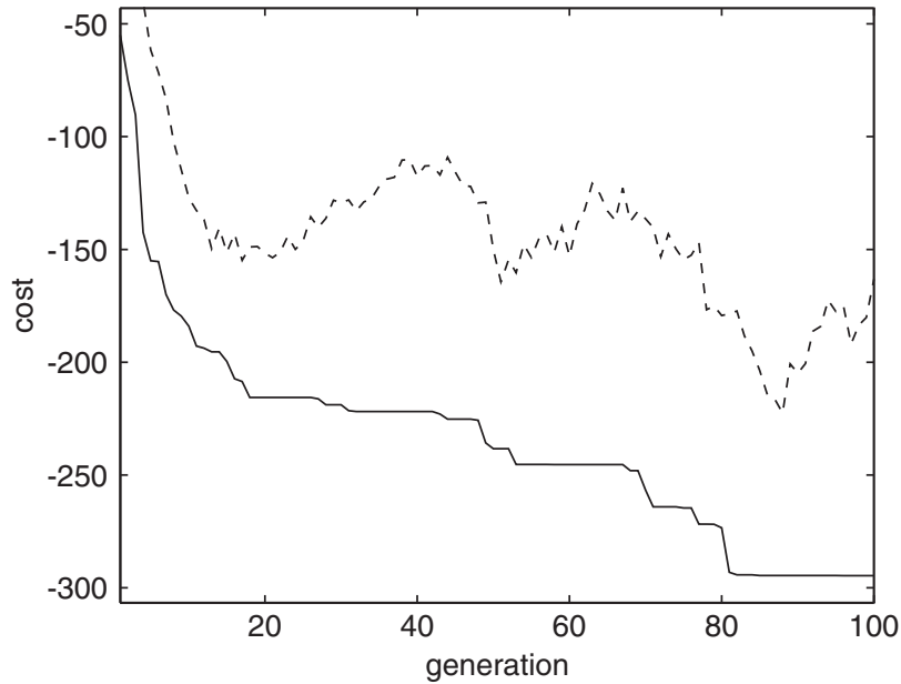
Figure 4.17 Plot of the mean (dashed) and minimum (solid) of the population as a function of generation for the continuous parameter GA applied to the antenna design problem.
