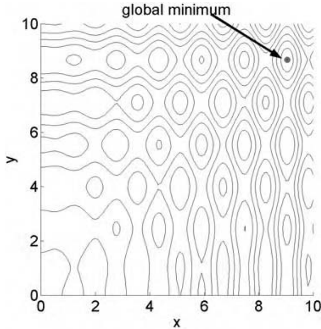
Figure 1.4 Contour plot of (1.1).
