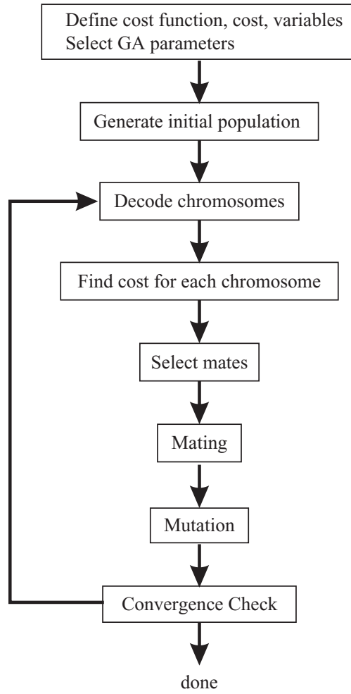
Figure 2.2 Flowchart of a binary GA.
